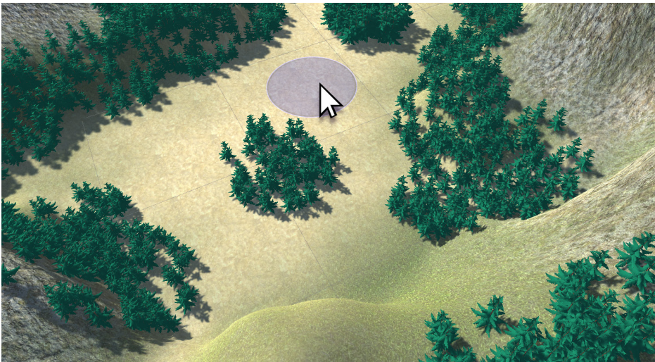
Figure 13.27: Our World Map, now covered in forests by using the Paint Trees tool.
