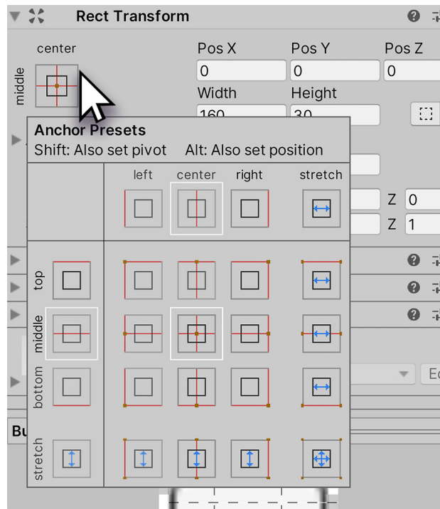
Figure 4.3: Anchors give you control over the relative placement of UI elements: very useful for building resolution-independent interfaces.
