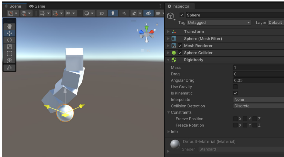
Figure 6.4: Our sphere object easily pushes around our chain of joint objects.
