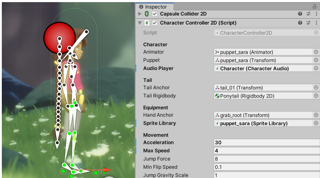
Figure 15.24: Just like our 3D hero, this 2D character has a Collider object and a custom made Controller script to handle movement of the Character.
