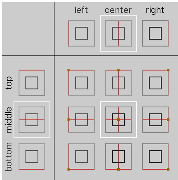
Figure 4.12: Anchor Presets determine which side of the parent this UI Element snaps to.
