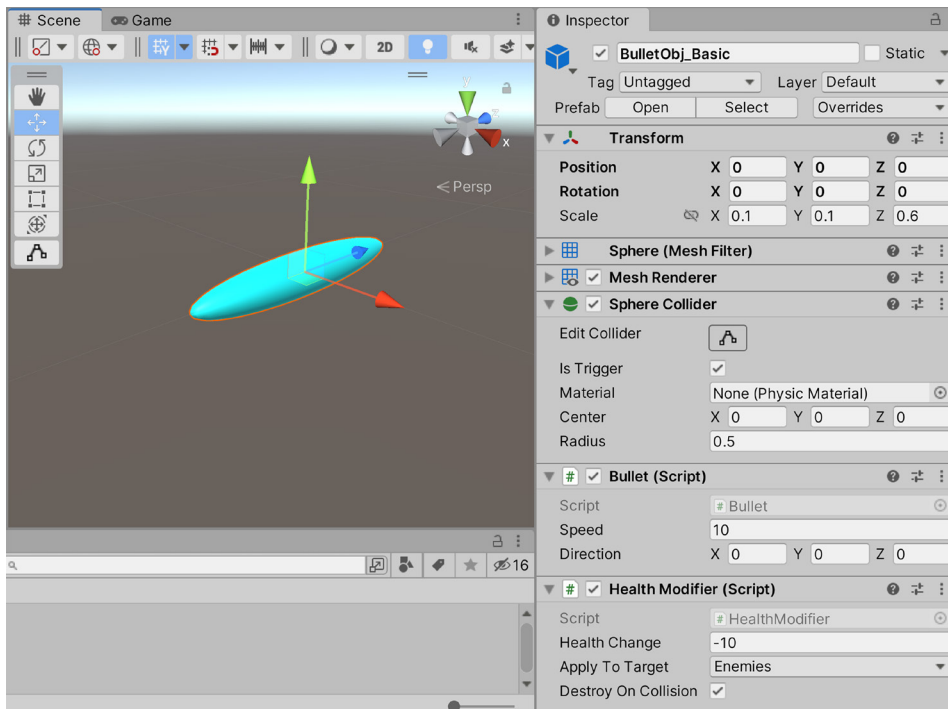
Figure 3.18: Our finalized Bullet prefab.
