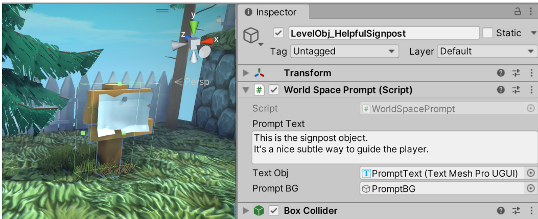
Figure 14.17: Our finalized Signpost, with Box Collider and our newly created Prompt script.
