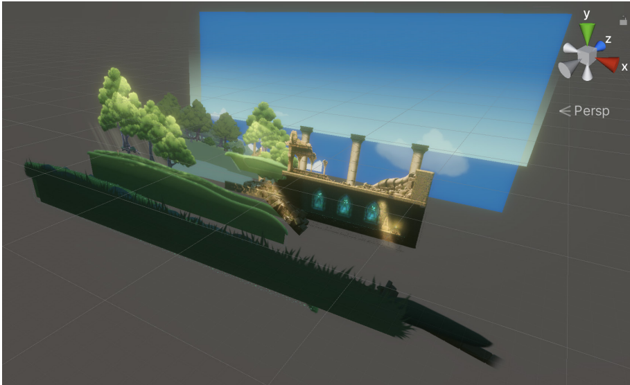
Figure 15.33: You can mimic the Parallax effect by moving distant objects further back in the scene.
