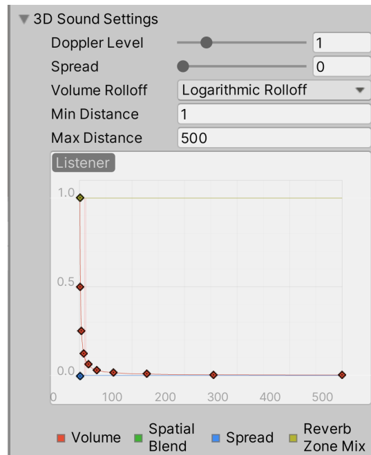
Figure 10.16: The 3D Sound Settings for this Audio Source.
