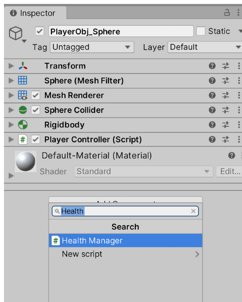
Figure 3.2: Use the Add Component “Search Bar” to quickly find our HealthManager component.
