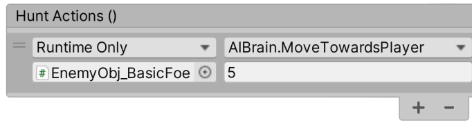
Figure 8.10: When Hunting the player, the only thing on the mind of the Basic Foe is moving towards the player at a speed of 5 units per second.
