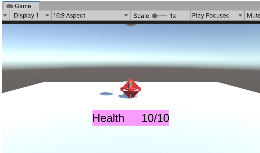
Figure 4.27: In the Game View window, your Current Health container should now look like this.
