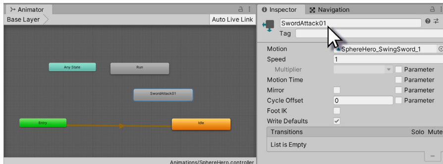
Figure 9.14: Rename our new animation SwordAttack01 . Our goal: any object that equips a sword, and has a 'SwordAttack01' animation clip, will play the proper animation when the attack button is pressed.
