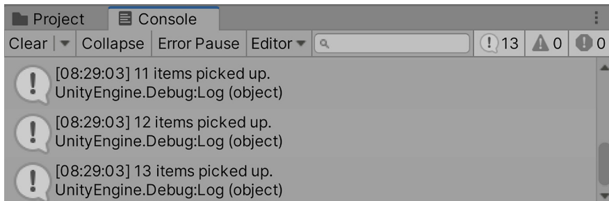
Figure 2.16: The debug console shows you Messages, Warnings, and Errors related to your game.
