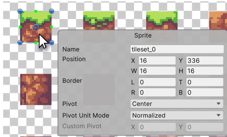
Figure 15.11: A successful slicing of our sprites. Our tilesheet is now ready for use in a Tilemap!
