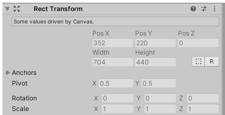
Figure 4.5: Position, size, rotation, and anchor parameters of a Canvas object.
