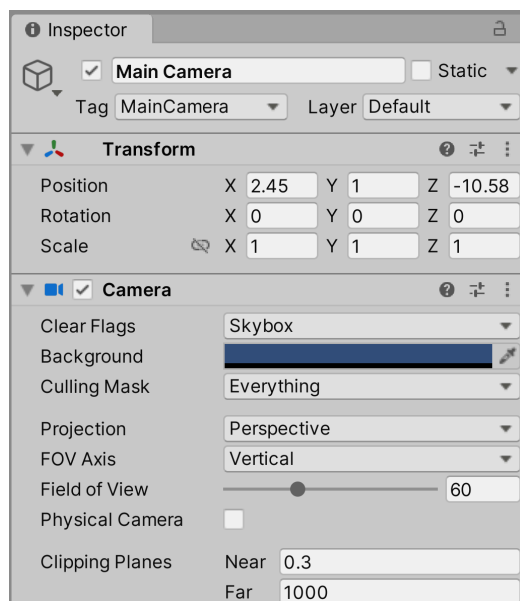
Figure 1.17: The Camera Inspector
