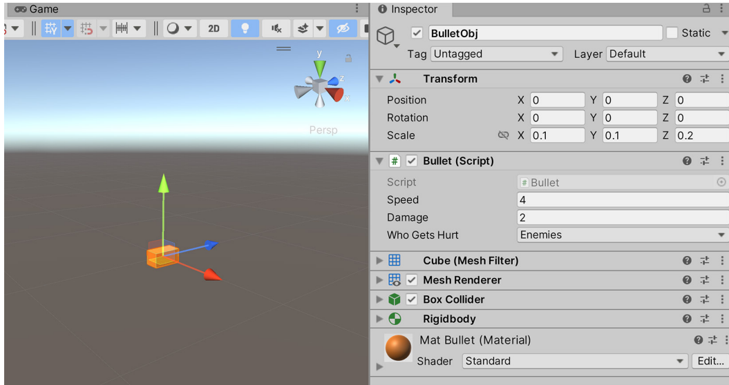
Figure 2.3: The Bullet is the simplest example: only having one unique script - “Bullet” - attached to it.
