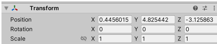
Figure 1.22: Transform panel
