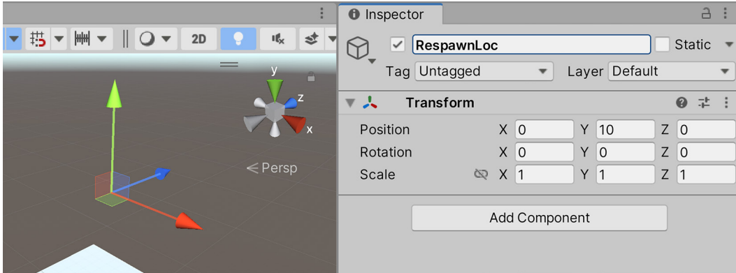
Figure 3.21: This empty GameObject represents the location that the player will respawn.
