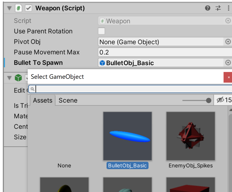
Figure 9.11: Assign the bullet prefab we want to spawn when firing this weapon.
