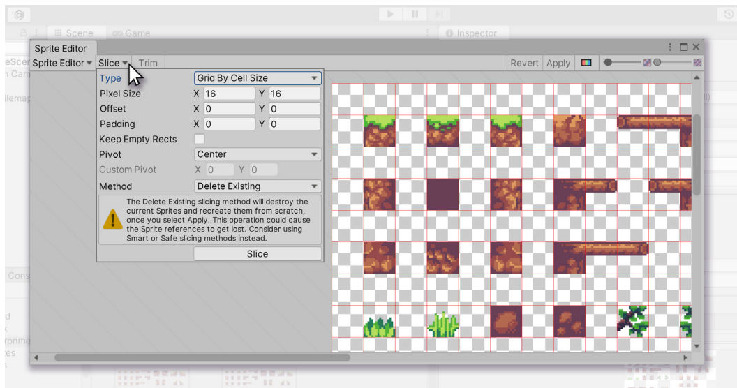
Figure 15.10: Unity can automatically Slice and Organize the sprites in your tilesheet.
