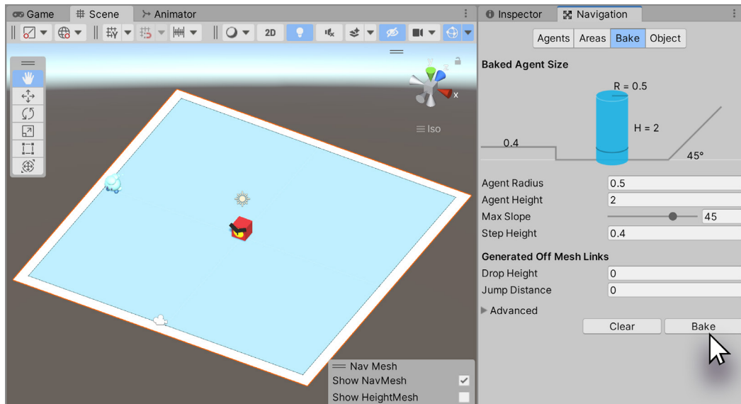
Figure 8.11: The generated NavMesh will appear as a blue, semi-transparent plane over your level geometry.
