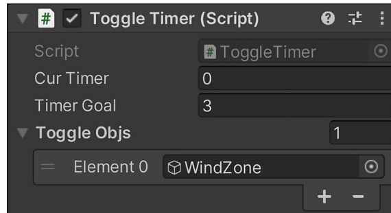
Figure 6.18: We've designed the Toggle Timer to contain a list of objects that it will turn on, then off, every X seconds.
